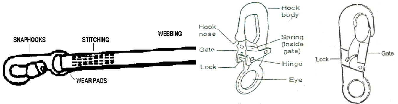
Figure 1n Snaphook, Self-locking
